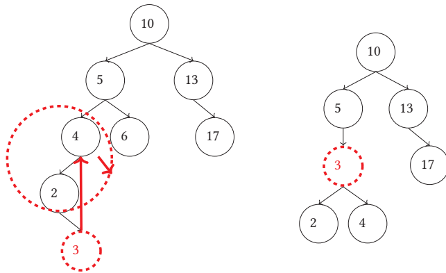
FIGURE 17 – Insertion de la clé 3
