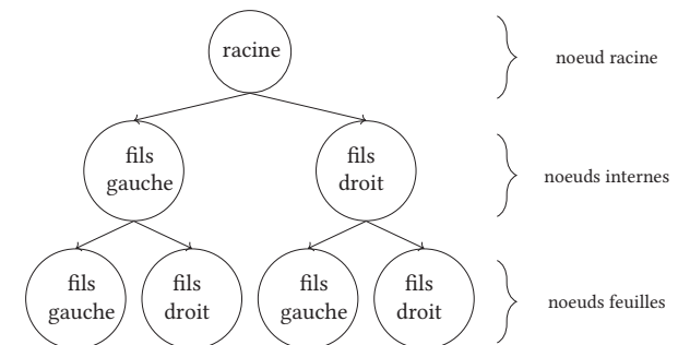
FIGURE 8 – Arbre
