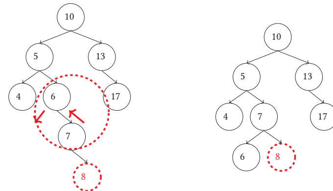
FIGURE 16 – Insertion de la clé 8
