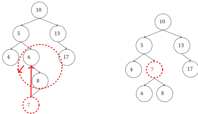
FIGURE 18 – Insertion de la clé 7
