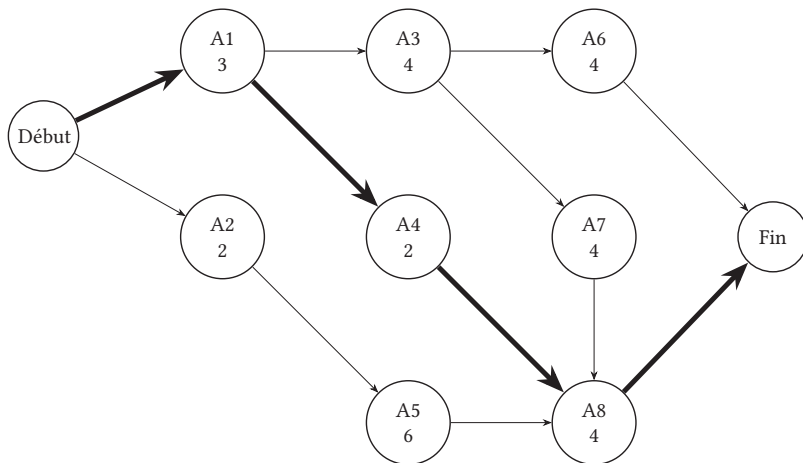
FIGURE 7 – Graphe
